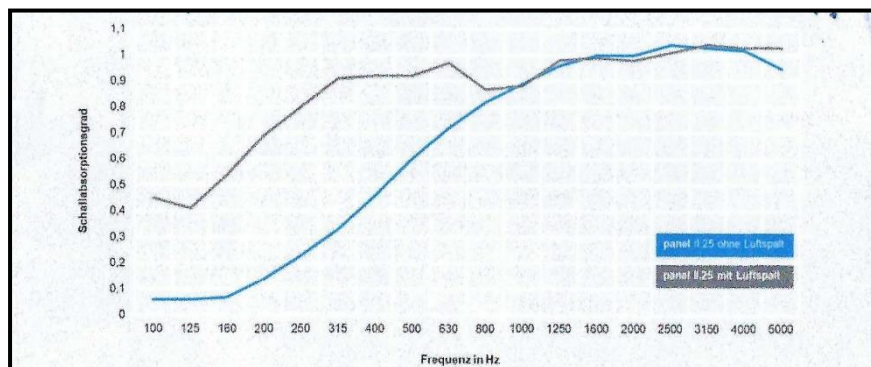
Luftschallabsorption 25 mm
